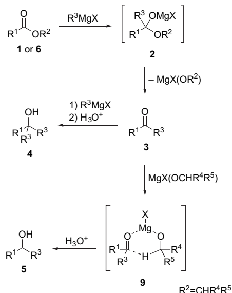
Scheme 3. Possible reaction mechanism.
