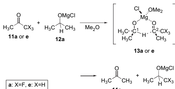
Figure 1. Transition state structure of 11 .
